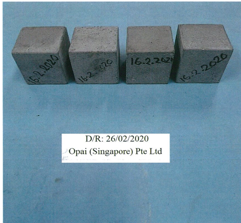
Photo. Four (4) pieces of 50mm x 50mm x 50mm thick Glass Fibre Reinforced Concrete (GFRC) cubes were received on 26/02/2020
